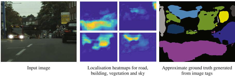
Fig. 3. Approximate ground truth generated from image-level tags using weak localisation cues from a multi-label classification network. Cluttered scenes from Cityscapes with full “stuff” annotations makes weak localisation more challenging than Pascal VOC and ImageNet that only have “things” labels. Black regions are labelled “ignore”. Colours follow Cityscapes convention.
