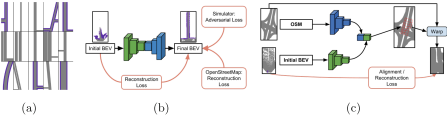
Fig. 4. (a) Simulated road shapes in the top-view. (b) The refinement-CNN is an encoder-decoder network receiving three supervisory signals: self-reconstruction with the input, adversarial loss from simulated data, and reconstruction loss with aligned OpenStreetMap (OSM) data. (c) The alignment CNN takes as input the initial BEV map and a crop of OSM data (via noisy GPS and yaw estimate given). The CNN predicts a warp for the OSM map and is trained to minimize the reconstruction loss with the initial BEV map.
