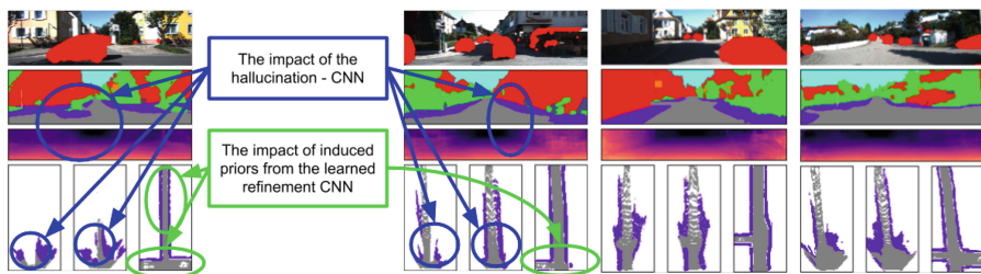
Fig. 7. Examples of our BEV representation. Each one shows the masked RGB input, the hallucinated semantics and depth, as well as three BEV maps, which are (from left to right), The BEV map without hallucination, with hallucination, and after refinement.
