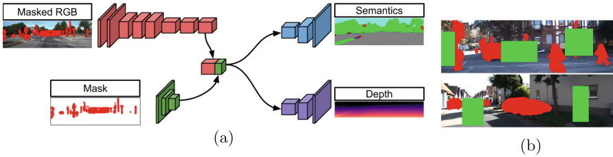
Fig. 2. (a) The inpainting CNN first encodes a masked image and the mask itself. The extracted features are concatenated and two decoders predict semantics and depth for visible and occluded pixels. (b) To train the inpainting CNN we ignore foreground objects as no ground truth is available (red) but we artificially add masks (green) over background regions where full annotation is already available
