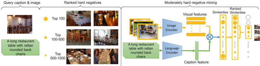
Fig. 3. Moderately hard negative mining. The left part shows a ground-truth caption and its top hard negatives mined from unlabeled images. The right part shows the process of moderately hard negative mining. The circles of different sizes stand for the similarities between each image and the query caption.
