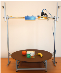
Fig. 2. The D2S image acquisition setup. Each scene was rotated ten times using a turntable. For each rotation, three images under different illuminations were acquired
