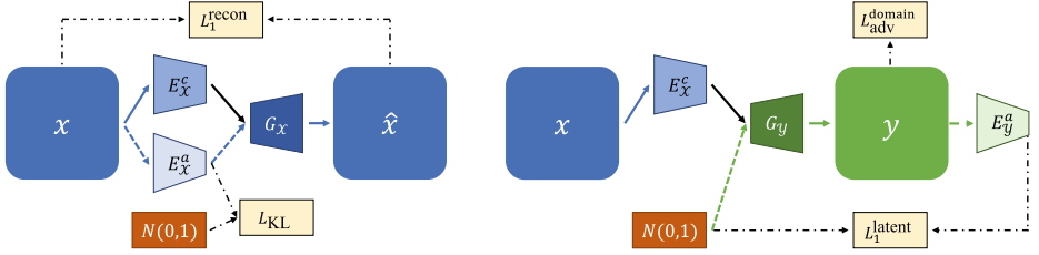
Fig. 4. Loss functions. In addition to the cross-cycle reconstruction loss L_1^{cc} and the content adversarial loss L_{adv}^{content} described in Fig. 3, we apply several additional loss functions in our training process. The self-reconstruction loss L_1^{recon} facilitates training with self-reconstruction; the KL loss L_{KL} aims to align the attribute representation with a prior Gaussian distribution; the adversarial loss L_{adv}^{domain} encourages G to generate realistic images in each domain; and the latent regression loss L_1^{latent} enforces the reconstruction on the latent attribute vector. More details can be found in Sect. 3.3.
