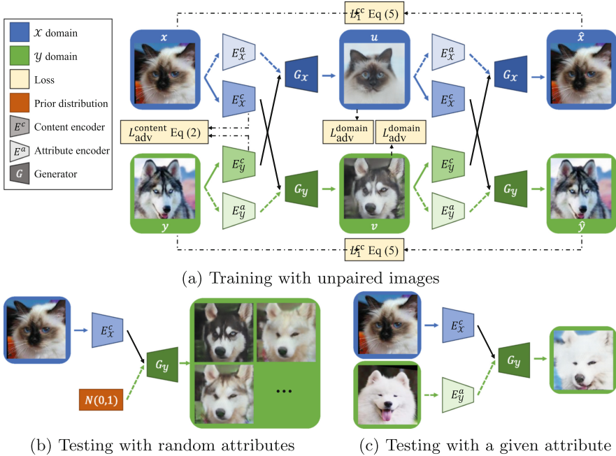
Fig. 3. Method overview. (a) With the proposed content adversarial loss L_{\text{adv}}^{\text{content}} (Sect. 3.1) and the cross-cycle consistency loss L_1^{\text{cc}} (Sect. 3.2), we are able to learn the multimodal mapping between the domain \mathcal{X} and \mathcal{Y} with unpaired data. Thanks to the proposed disentangled representation, we can generate output images conditioned on either (b) random attributes or (c) a given attribute at test time.
