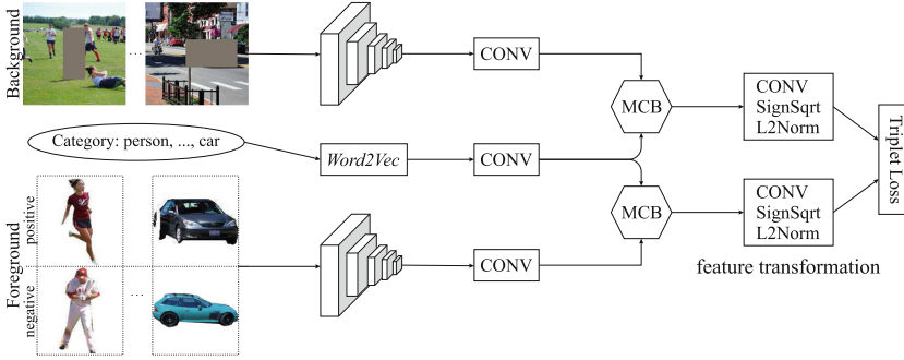
Fig. 2. Overall framework of the proposed compositing-aware image search (CAIS) system. A symmetric two-stream feature embedding network is utilized to extract background and foreground image features separately, in which a MCB module is introduced to incorporate category information. A feature transformation module is then performed to generate the final feature representations.
