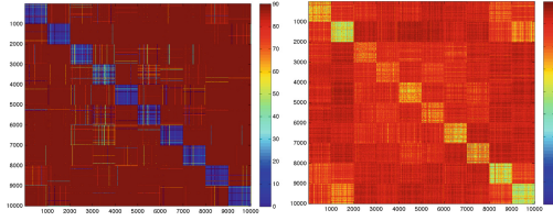
Fig. 3. Angles between the deep features learned for the validation set of CIFAR-10 using VGG-16. (Left) with additional low-rank loss. (Right) with the standard softmax loss. With low-rank loss, the intra-class variations among features are collapsed and inter-class features are orthogonal, which are particularly preferred at each tree split node.
