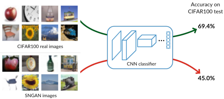
Fig. 1. State-of-the-art GANs, e.g., SNGAN [36], generate realistic images, which are difficult to evaluate subjectively in comparison to real images. Our new image classification accuracy-based measure (GAN-train is shown here) overcomes this issue, showing a clear difference between real and generated images.
