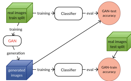
Fig. 2. Illustration of GAN-train and GAN-test. GAN-train learns a classifier on GAN generated images and measures the performance on real test images. This evaluates the diversity and realism of GAN images. GAN-test learns a classifier on real images and evaluates it on GAN images. This measures how realistic GAN images are.
