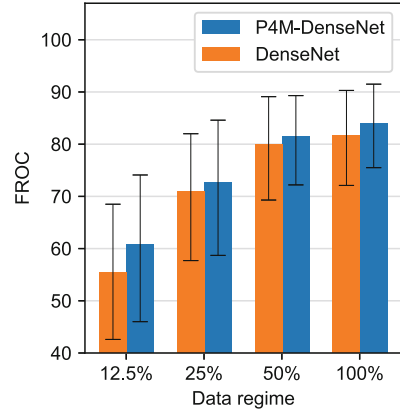
Fig. 4. Performance on the Camelyon16 test set. The confidence bounds are obtained using a 2000-fold bootstrap regime. *Challenge winner [17] uses 40\times resolution and is not directly comparable.
