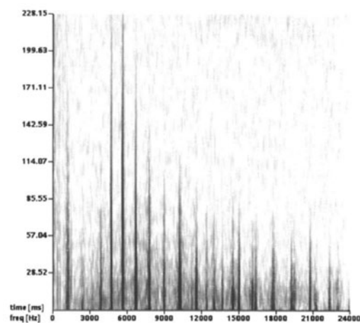
fig.4 Spectrum of the real sound
