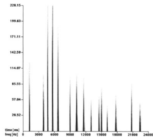
fig.5 Spectrum of the synthesized sound
