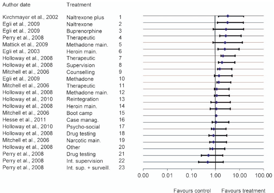
Fig. 8.1 Forest plot of weighted mean ORs by review. (Figure sorted by OR (highest to lowest))
