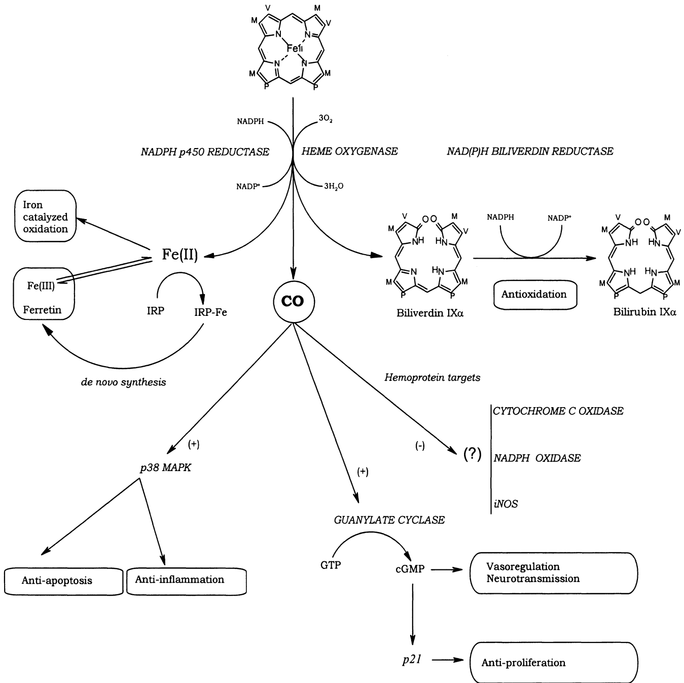
Fig. 1. Functional consequences of HO activity. Heme oxygenase degrades heme to biliverdin-IX \alpha , carbon monoxide, and iron. Biliverdin-IX \alpha is converted to bilirubin-IX \alpha by NAD(P)H biliverdin reductase. Both bile pigments have potent in vitro antioxidant activity. Redox-active iron released from HO activity may promote oxidative damage. However, by inactivating iron regulatory protein (IRP) activity, iron stimulates the synthesis of ferritin, an iron-sequestration protein and possible cytoprotectant. CO derived from the HO reaction has possible significance in the regulation of vascular and neural functions. The stimulation of cGMP-dependent signal transduction pathways may account for the vasodilatory and anti-proliferative effects. CO has potent anti-inflammatory effects, which depend on downregulation of pro-inflammatory cytokine production mediated by modulation of p38 MAPK. The abbreviations used in this figure include: cGMP = guanosine 3',5'-cyclic monophosphate; CO = carbon monoxide; Fe(II) = ferrous iron; Fe(III) = ferric iron; GTP = guanosine triphosphate; IRP = iron regulatory protein; NOS = nitric oxide synthase; p38 MAPK = p38 mitogen activated protein kinase.
