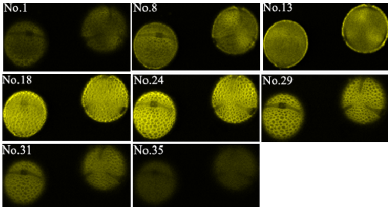
Fig.1. A series of confocal microscope digital images of Weeping Forsythia pollen. Pollen was labeled with AO. Thirty-five images were acquired with the laser-scanning confocal microscope, and eight images (from No.1 image to No.35 image) were chosen in the figures. ( \times 400 ).
