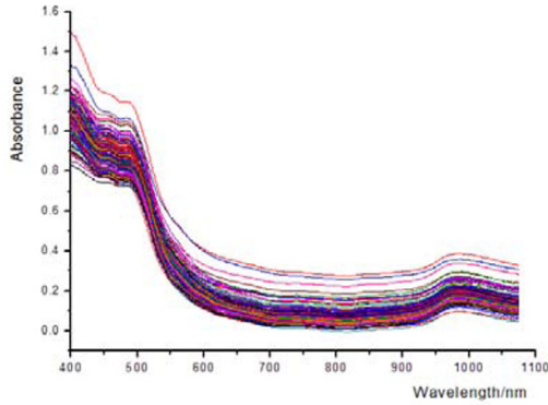
Figure 1. Whole Absorbance spectra of mango
