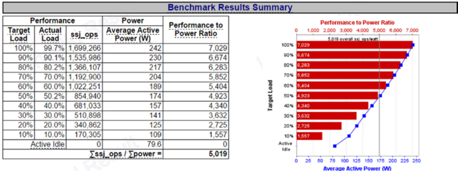
Figure 1-5. A sample of a SPECpower published result. The table emphasizes both workload performance and energy efficiency
