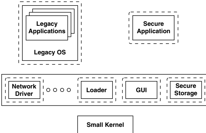
Figure 2. Nizza architecture.
