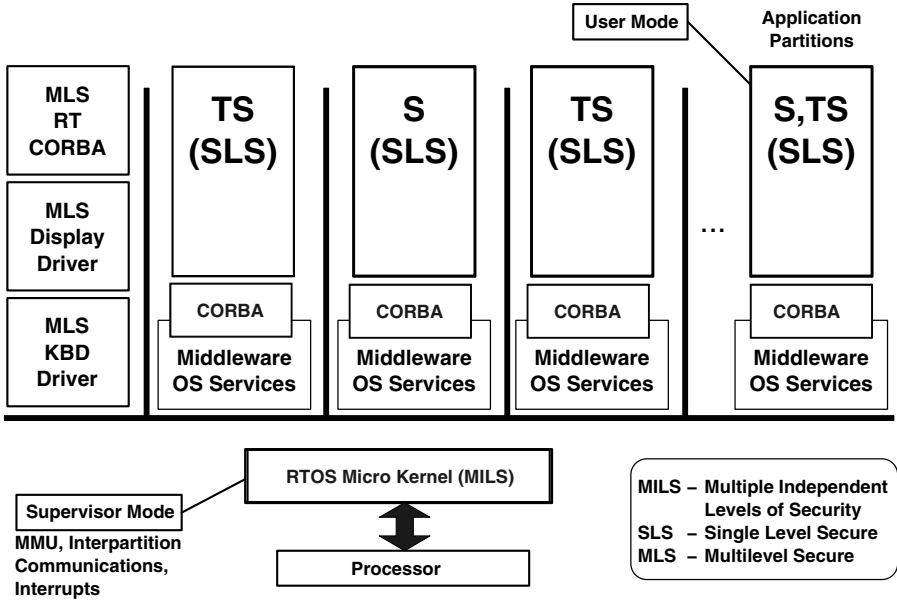
Figure 1. MILS architecture.
