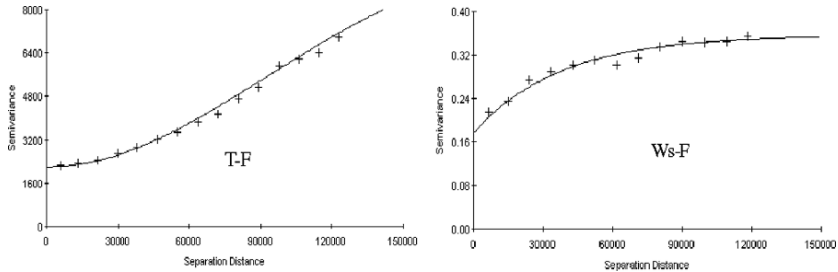
Fig. 4. Experimental semivariograms of soil fluoride element with fitted models
