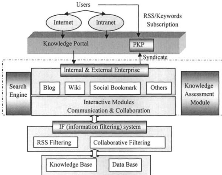
Fig. 3 Framework of a Web2.0-based Knowledge Management Platform
