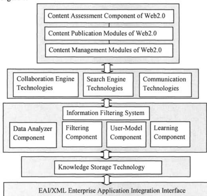
Fig. 4 Technology Architecture of a Web2.0-based KM Platform
