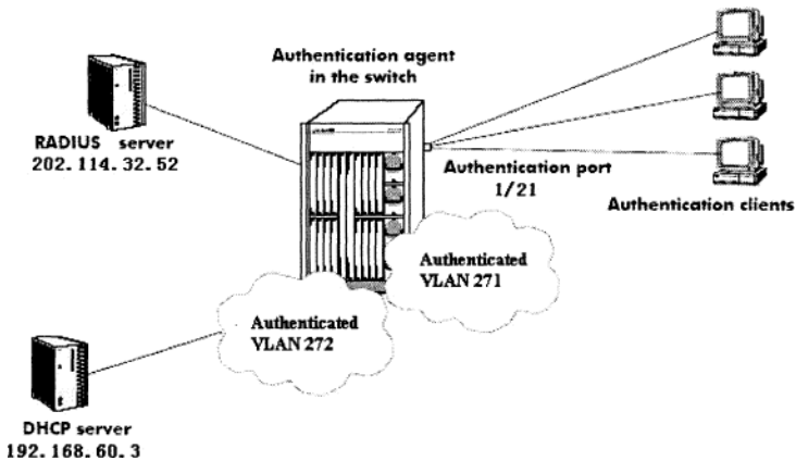
Fig. 1. HTTP Authenticated Network Components
