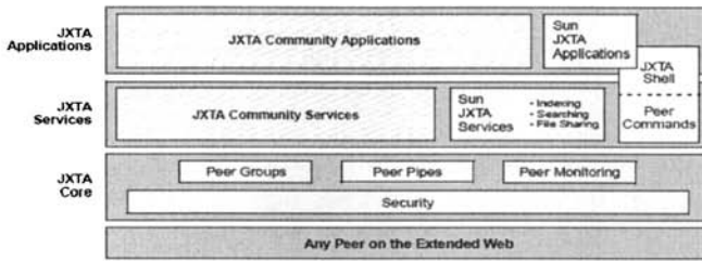
Fig. 1. P2P Software Architecture
