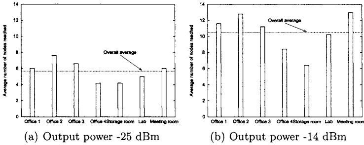
Fig. 3. Average number of nodes reached by coordinate message broadcasts
