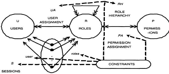
Figure 1. RBAC 3 model.
