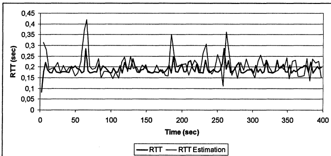
Figure 2. RTT Estimations
