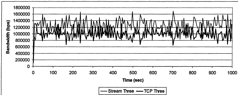
Figure 6. Bandwidth distribution on C1-C4 bottleneck link
