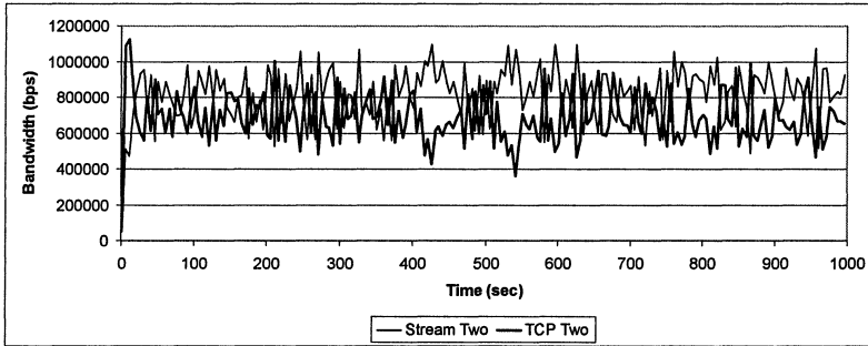
Figure 5. Bandwidth distribution on C1-C3 bottleneck link
