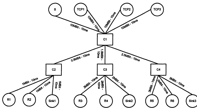
Figure 3. Topology with no share links
