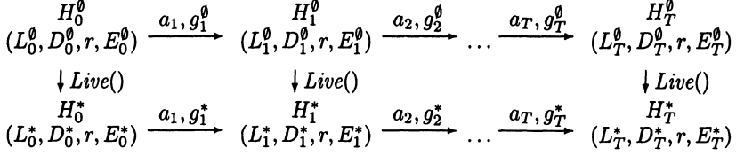
Figure 2. Expanded Program History, including the null ( H^\emptyset ) and reachable ( H^* ) heap states.
