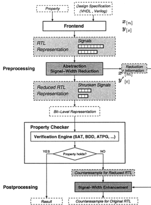
Figure 1. Property Checking Flow
