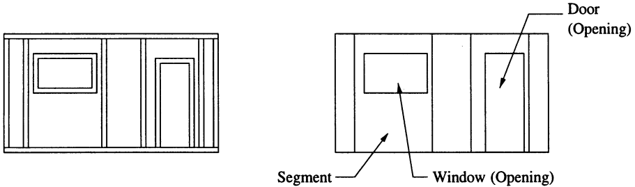
Figure 3.3 Structure of a wall.
