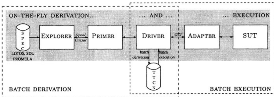
Figure 1 TORX tool architecture
