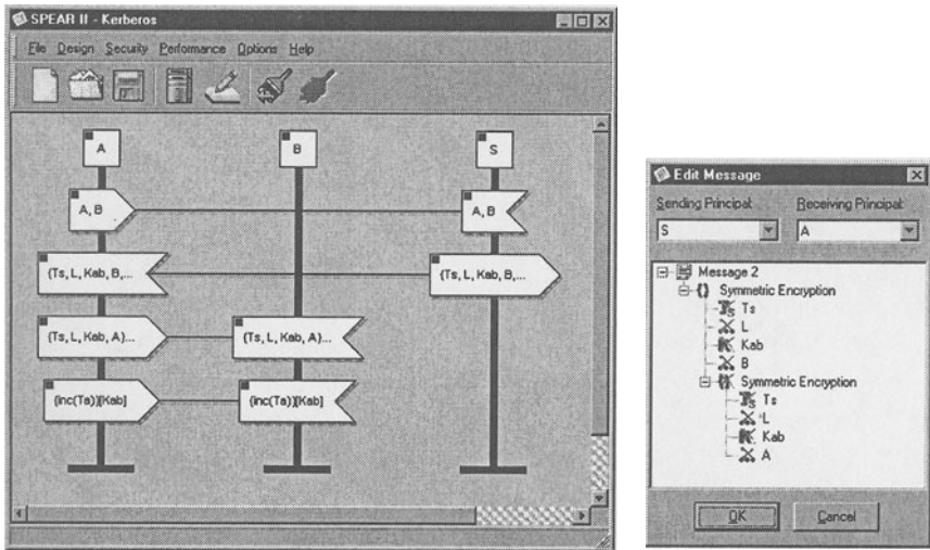
Figure 1 An illustration of the high-level protocol view on the left and the component view on the right, as implemented in the SPEAR II tool.
