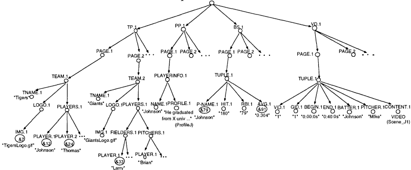
Figure 17 Tree representation of the source data.
