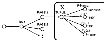
Figure 20 An object set X such that (\forall o_i \forall o_j \in X) Share_{BS.1 \rightarrow PAGE.?\rightarrow TUPLE.1}(o_i, o_j) .
