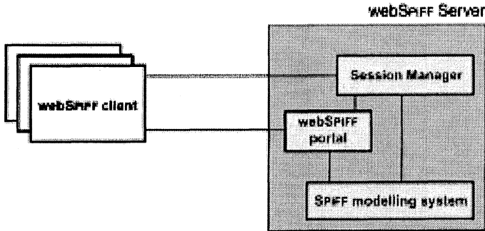
Figure 1. Architecture of webSPIFF
