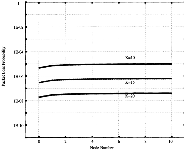
Fig.10 Packet loss probabilities at nodes
