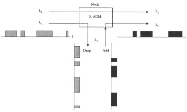
Fig. 1(a) Wavelength add/drop multiplexer ( \lambda -ADM)
