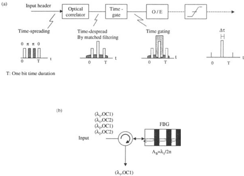
Fig.5 (a) Configuration of photonic code selector. (b) FBG-based optical correlator
