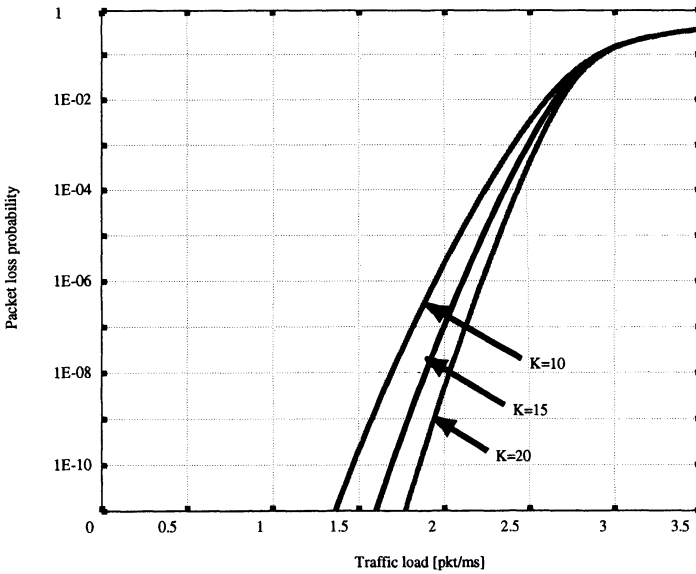
Fig.11 Packet loss probabilities vs. traffic load
