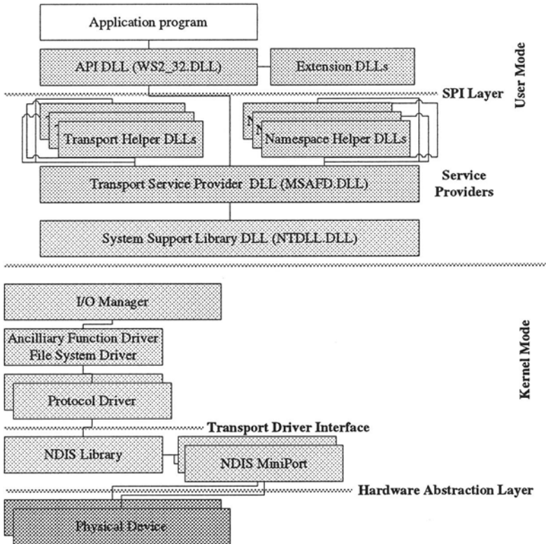
Figure 1 Interacting Components in WinSock Calls
