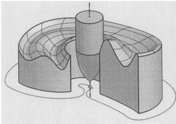
Figure 3: Milling a surface with boundary.
