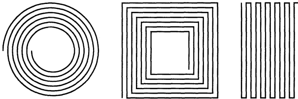
Figure 8: Milling path schemes.
