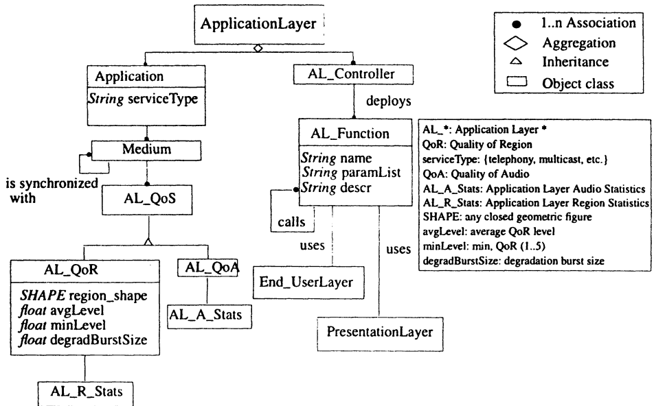
Figure 5 A modeling of QoS-related information at the application layer.
