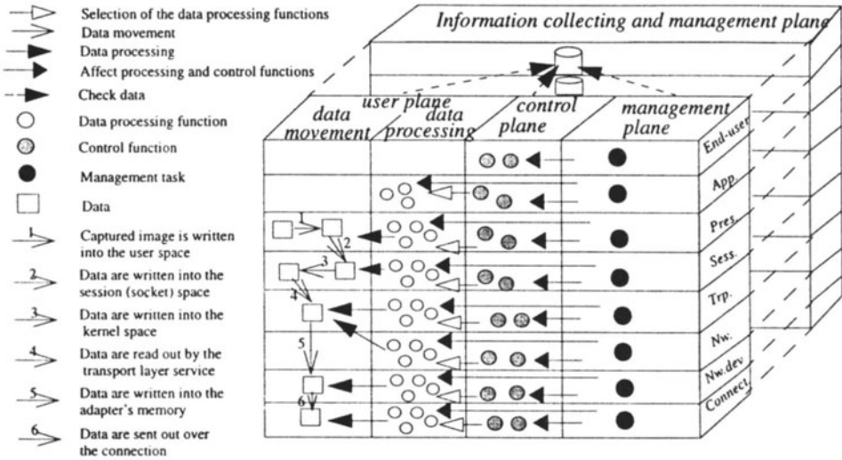
Figure 3 Interactions among the framework planes.
