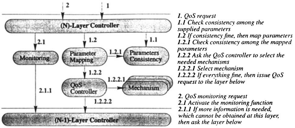
Figure 7 A processing model for control requests issued to layer (N).
