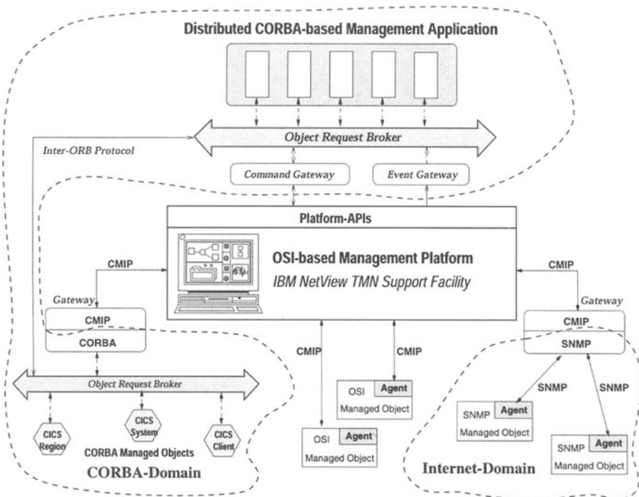
Figure 5 Interoperability between different management architectures
