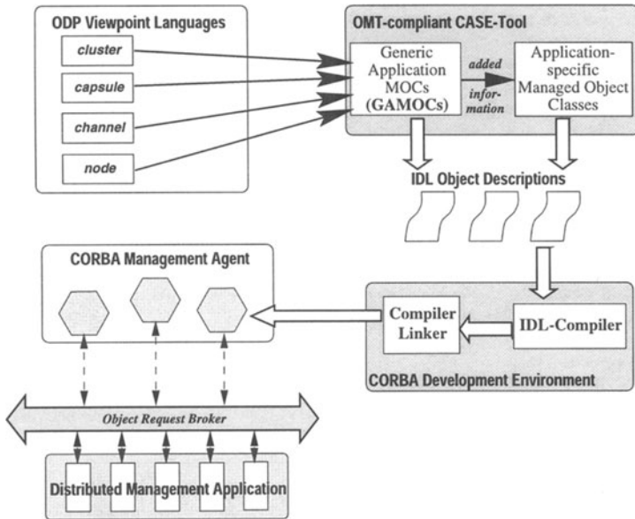
Figure 4 Overview of the transformation process
