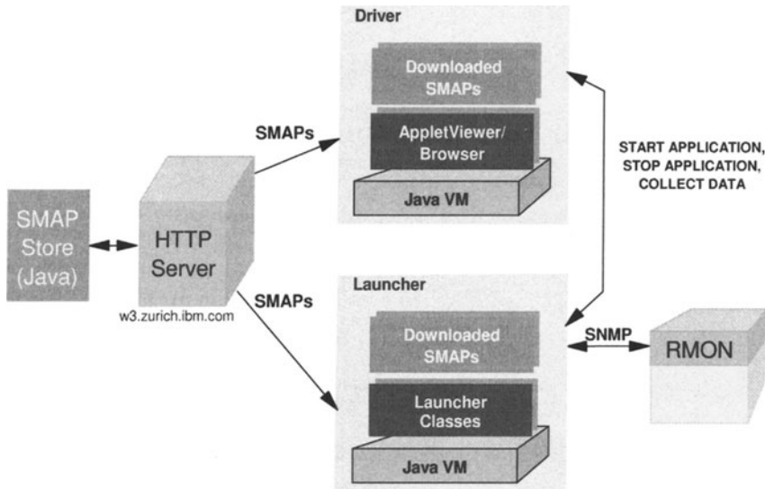
Figure 3 SMAP RMON Example
