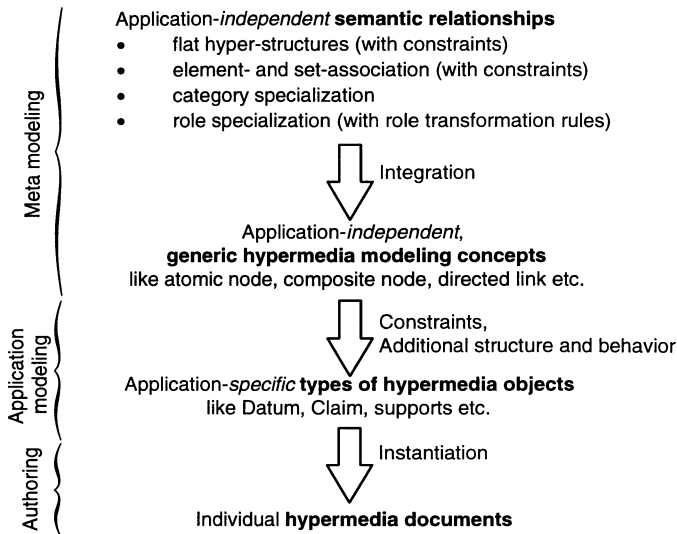
Figure 1 Overview of the approach followed in the design of the hypermedia engine.
