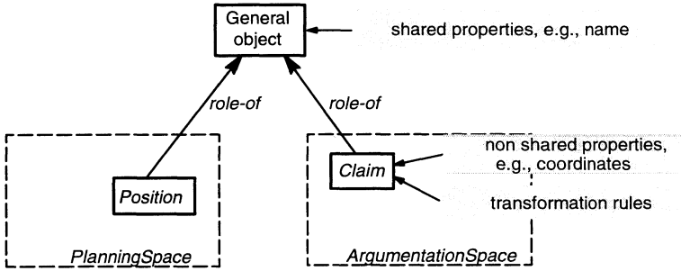
Figure 3 Example of the usage of role specialization.
