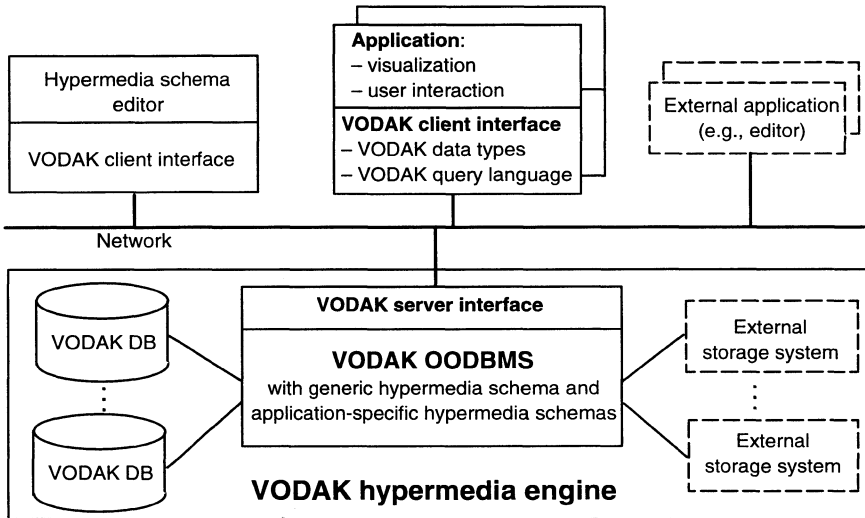
Figure 7 System architecture of the VODAK hypermedia engine.
