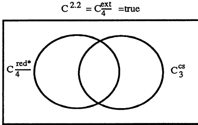
Figure 2: LOTOS Consistency Relations
