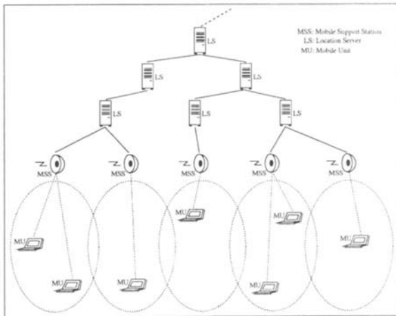
Figure 2. Location servers in the Mobile Network (after [1])
