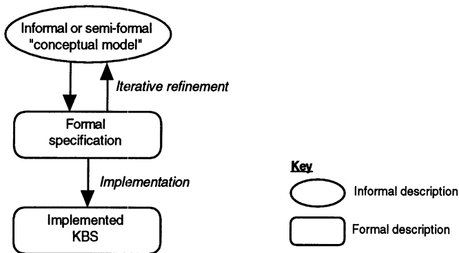
Figure 1 Using a formal specification in KBS development.
