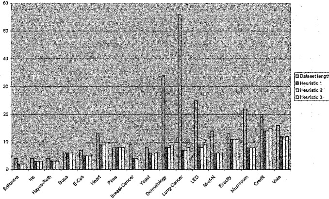
Figure 1 Reduction of the dataset length by RSReduce
