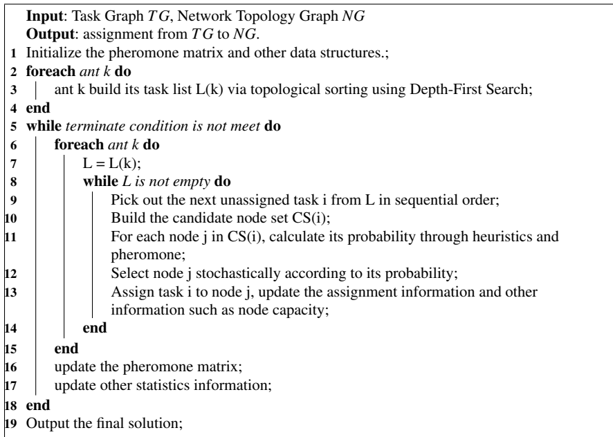
Fig. 1 The ANTS-TETA algorithm
