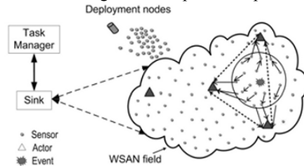
Fig. 1 Physical architecture of a WSAN [5]
