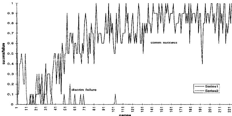
Figure 2. Graph showing the average failure in discrimination (series 2 on y-axis) against the number of discrimination games (x-axis - scale 1/10). The communicative success is shown as series 1.
