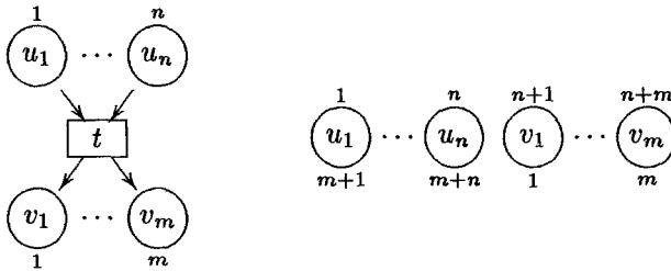
Figure 3: A transitions t_{u,v}: u \rightarrow v and the symmetry \gamma(u, v) in CQ[N]
