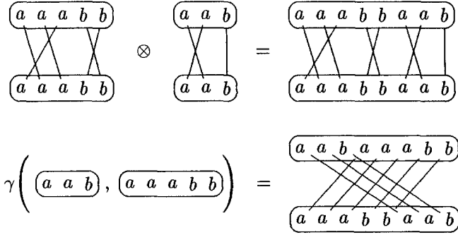
Figure 1: The monoidal structure of Sym_S^*
