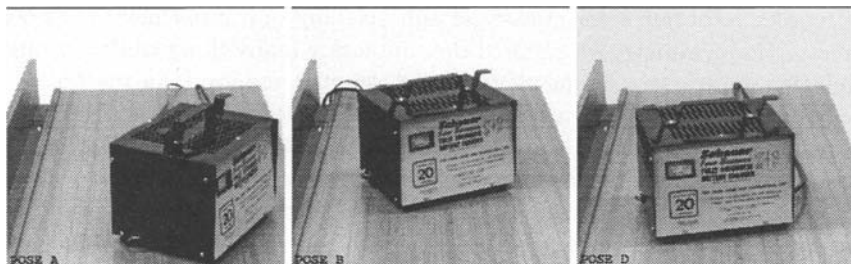
Fig. 5. Three 2D images of a 3D mirror-symmetric object from different view points.
