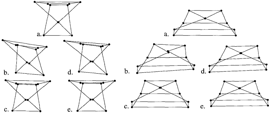
Fig. 4. Reconstruction of 3D mirror-symmetric configurations from noisy 2D projections - see text.
