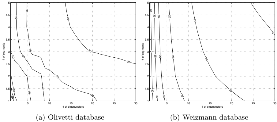
Fig. 2. Tradeoff between number of segments (the y-axis) and number of eigenvectors (the x-axis). The contour labels measure the reconstruction error (in intensity values) per pixel. For example, In the Olivetti database one segment with 21 eigenvectors has the same reconstruction error, for this image ensemble, as a 5-segment 5-eigenvector combination. See text for further details.
