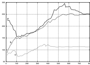
Fig. 5. Statistics: the graph represents the evolution of the number of vertices of the model with respect to the iteration number, and for different metrics. The segmented image is the same as in Fig. 4. This emphasizes that our new model is able to extract image components with significantly less vertices than the initial model, especially if anisotropic metrics are used (curve c on the graph). It also shows that the use of deformed metrics speeds up the model convergence. Computation times remain higher than with an Euclidean metric, however, many optimizations are likely to be performed to reduce the computational cost per vertex.
