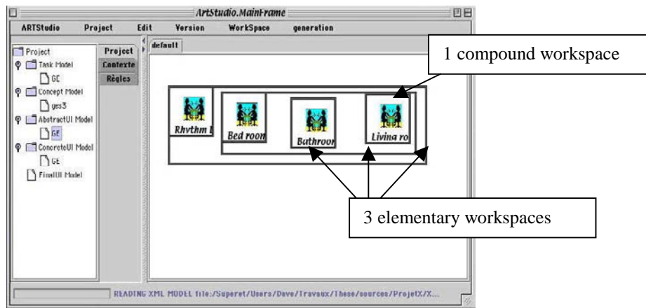
Fig. 11. The Abstract User Interface generated by ARTStudio from the Task Model of Figure 9. Thick line rectangles represent compound workspaces whereas thin line rectangles correspond to elementary workspaces.
