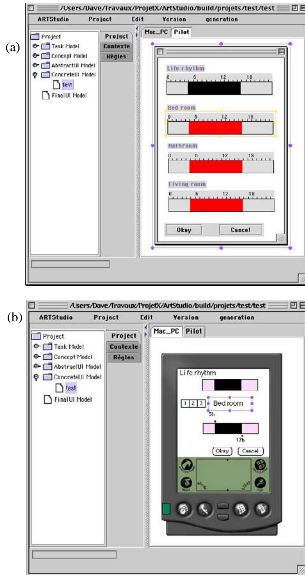
Fig. 13. In a), the concrete user interface generated for the system when running on the large screen display of Figure 1a. In b), the concrete user interface that corresponds to Figure 1b for the Palm Pilot.
