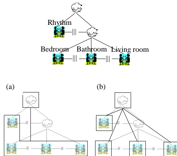
Fig. 12. ARTStudio allows the designer to reconfigure the relationships between workspaces.
