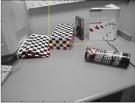
Fig. 1. (Left) A display of the real-time system. Selected features are highlighted by asterisks, and a virtual object (a reference frame) is placed in the scene. As the camera moves, the image of the virtual object is modified in real time, according to the estimated motion and structure of the scene, so as to make it appear stationary within the scene. Other displays visualize the motion of the camera relative to an inertial reference frame, and a bird's eye view of the reconstructed position of the points tracked. (Right) Structure error: the error in mutual distance between a set of 20 points for which the relative position is known (the squares in the checkerboard box on the left) are plotted for a sequence of 200 frames. Mean and standard deviation, both computed across the set of points at the last frame and across the last 100 frames, are below one millimeter. The experiment is performed off-line, and only unoccluded features are considered.
